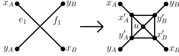
Figure 3: Replacement of the edge crossing with five new vertices and twelve new edges.
