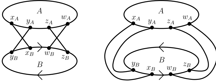
Figure 1: If |S'| = 2 , then vertical flipping of B gives a planar embedding.
