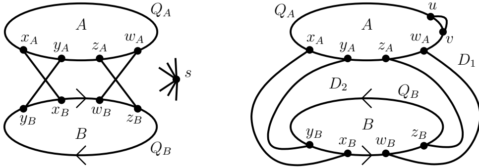
Figure 2: Vertical flipping of B in G - s to obtain the plane graph G'' .
